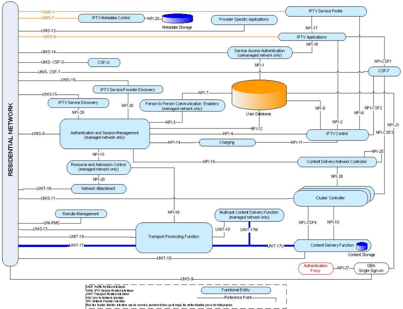
Figure 2: Provider Network High Level Architecture
