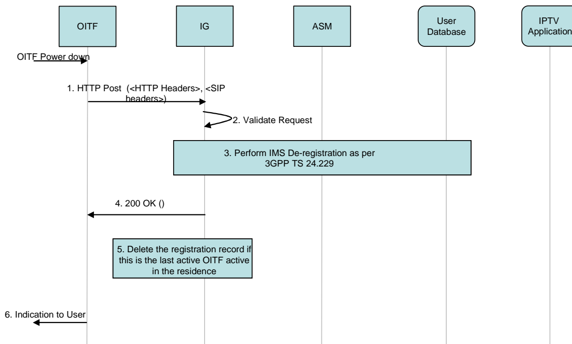
Figure 9: IPTV Default Identity De-registration procedure in a managed model
