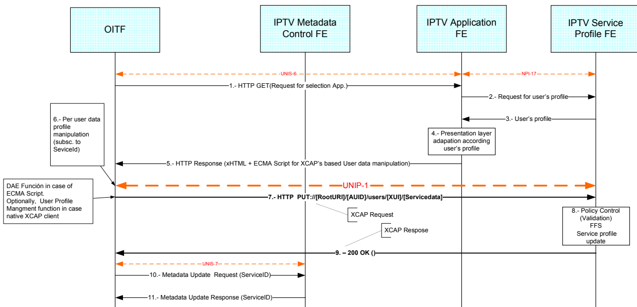
Figure 11: Service Profile Management Based on XCAP
