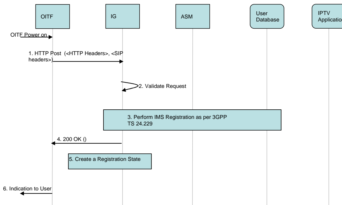
Figure 6: Default IMS Public identity Registration procedure in a managed model
