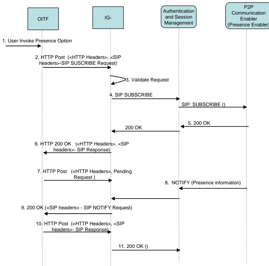
Figure 16: Subscription to Presence
