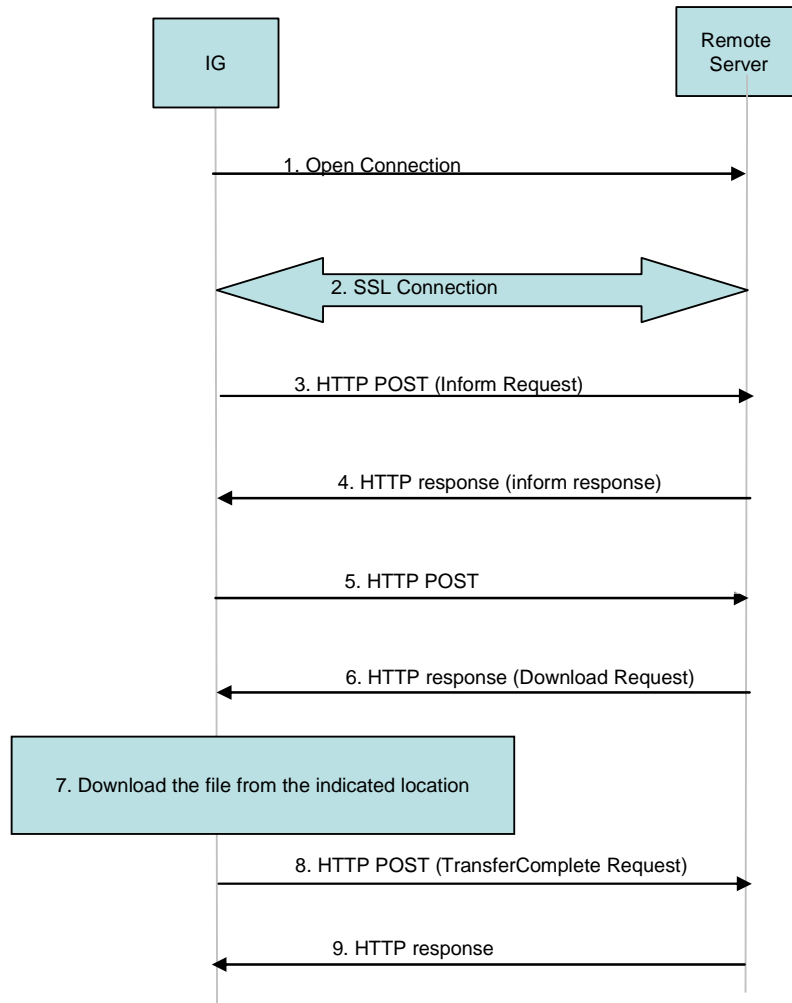
Figure 3: Sequence for the Configuration of an IG
