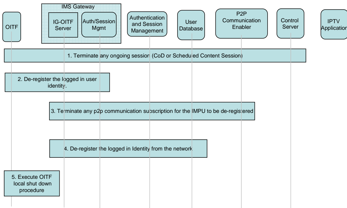
Figure 21: High level Shut-down procedural flow for an OITF
