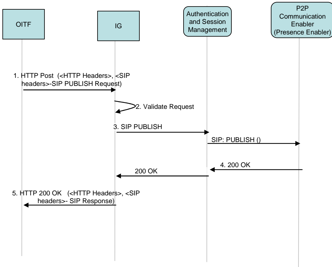
Figure 18: Publishing a Presence Event
