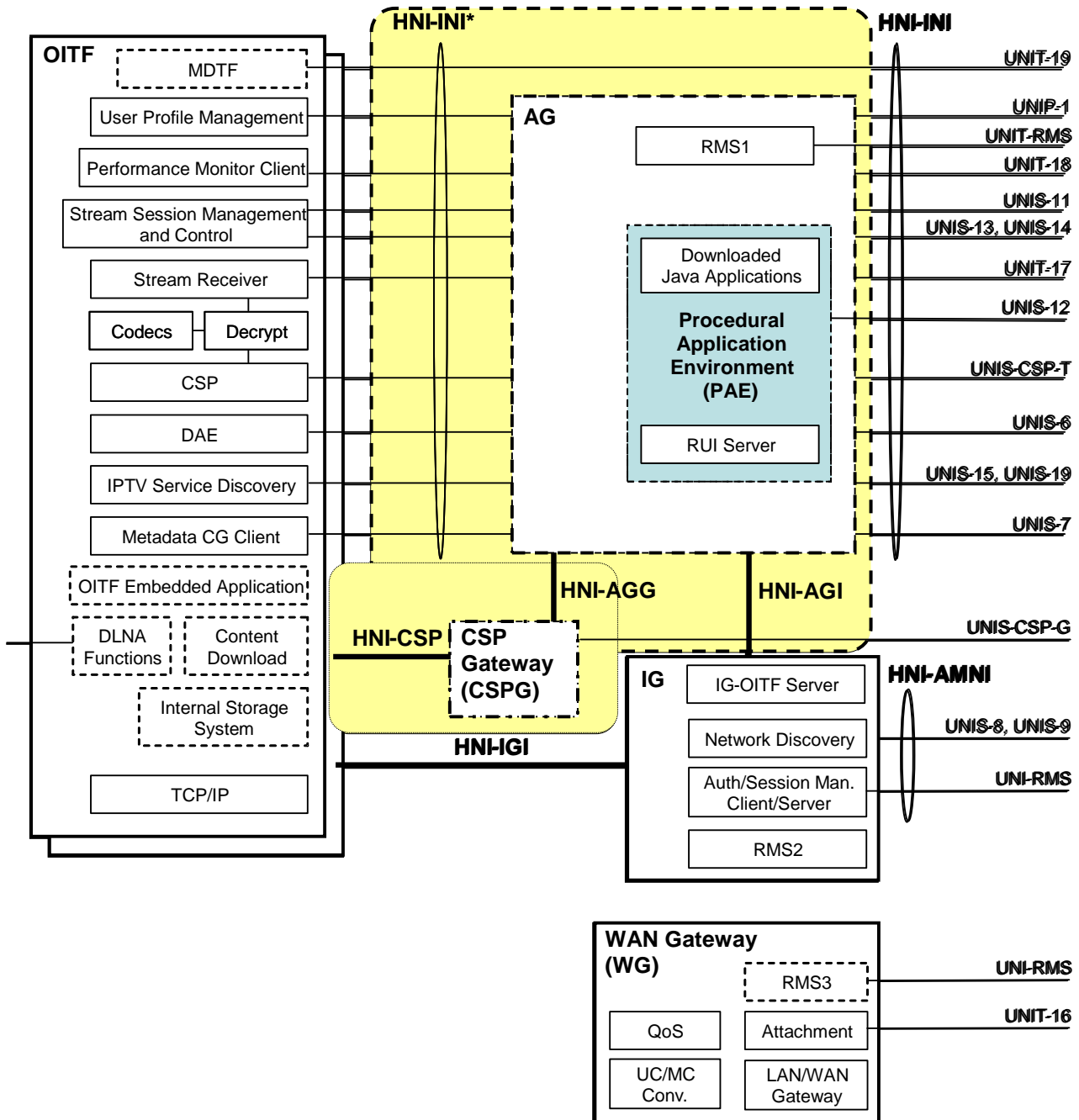
Figure 1: Consumer Network High Level Architecture
