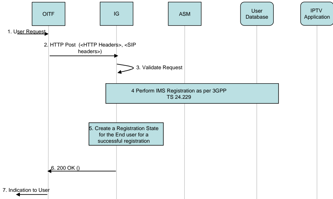
Figure 7: IPTV end-user IMPU Registration procedure in a managed model
