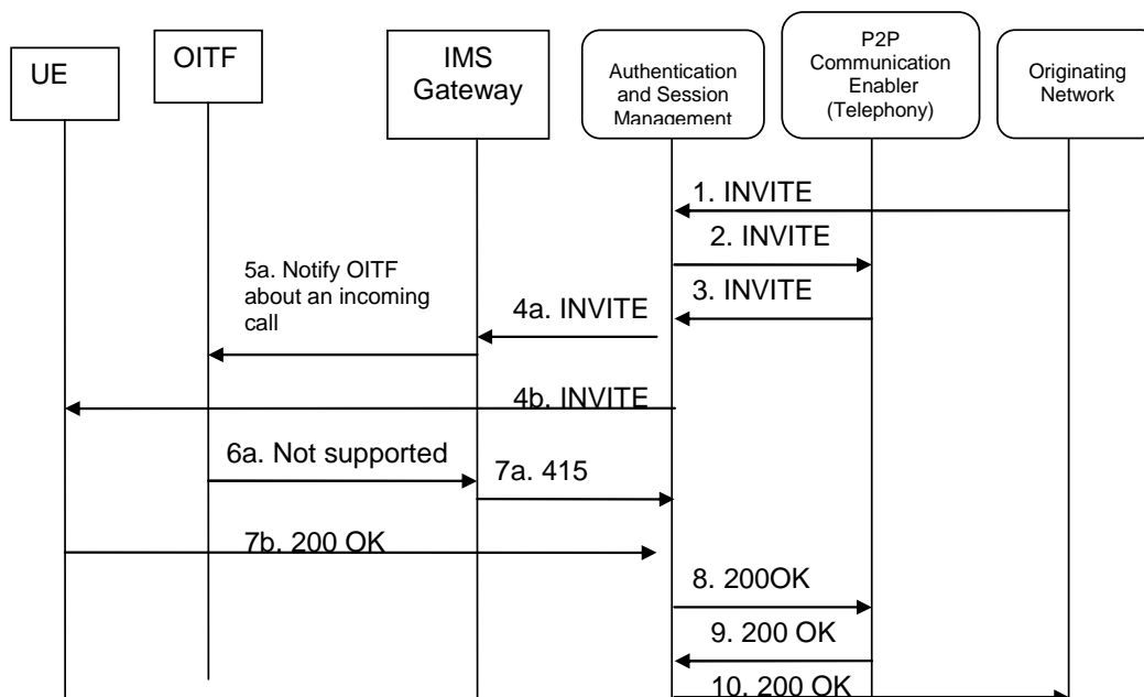
Figure 15: IMS telephony service based caller identification
