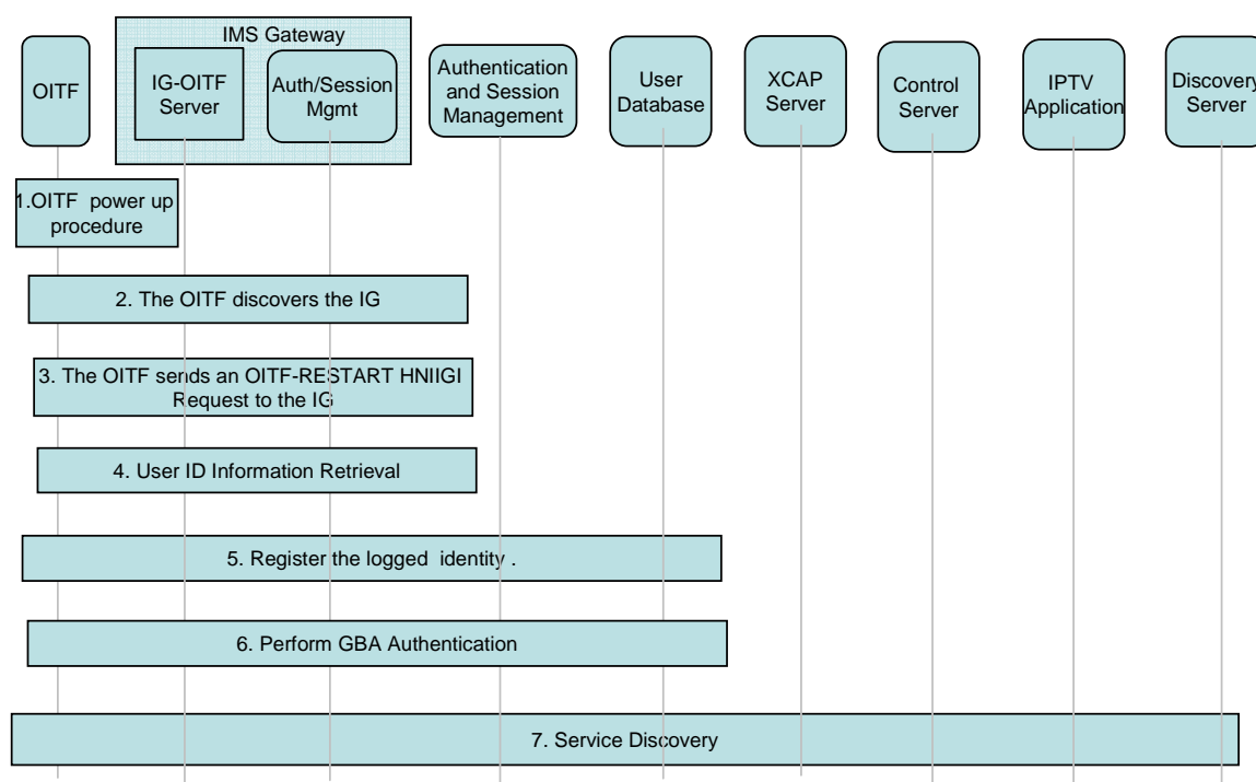
Figure 20: High level Start up procedural flow for an OITF
