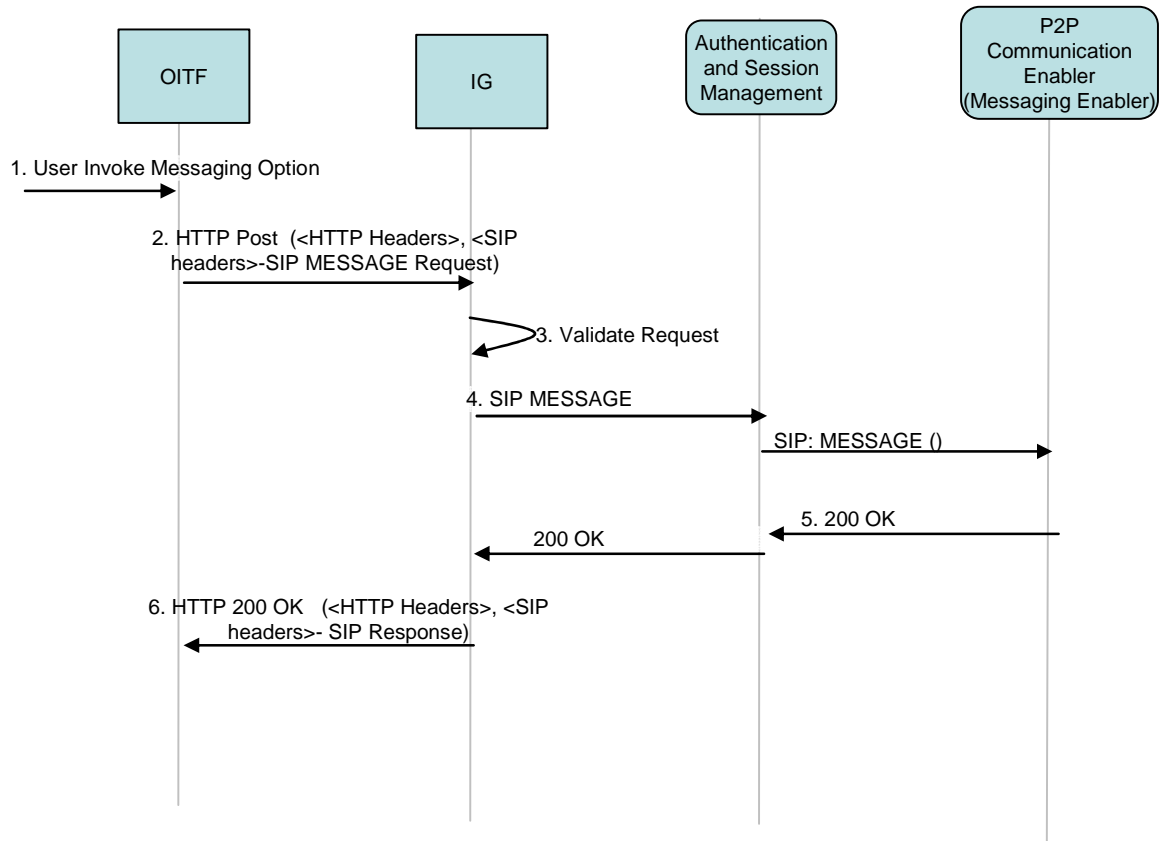
Figure 13: Instant Message Origination Call Flow
