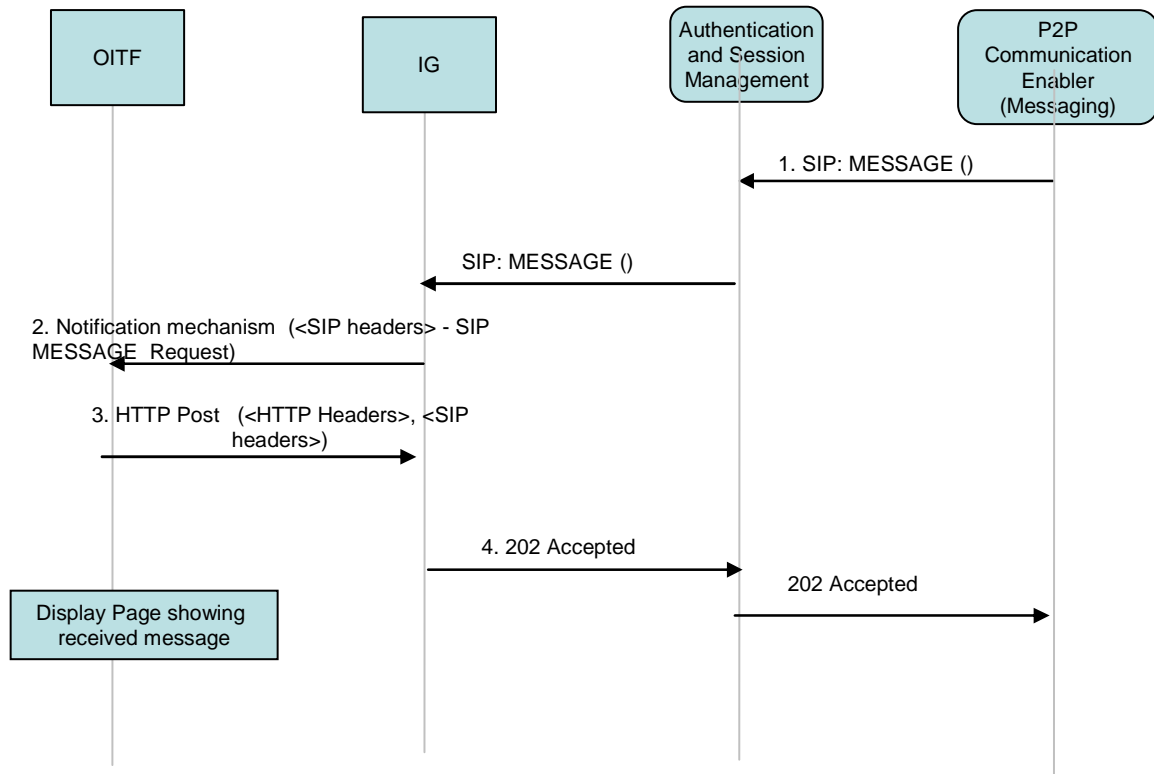
Figure 15: Caller identification Call Flow
