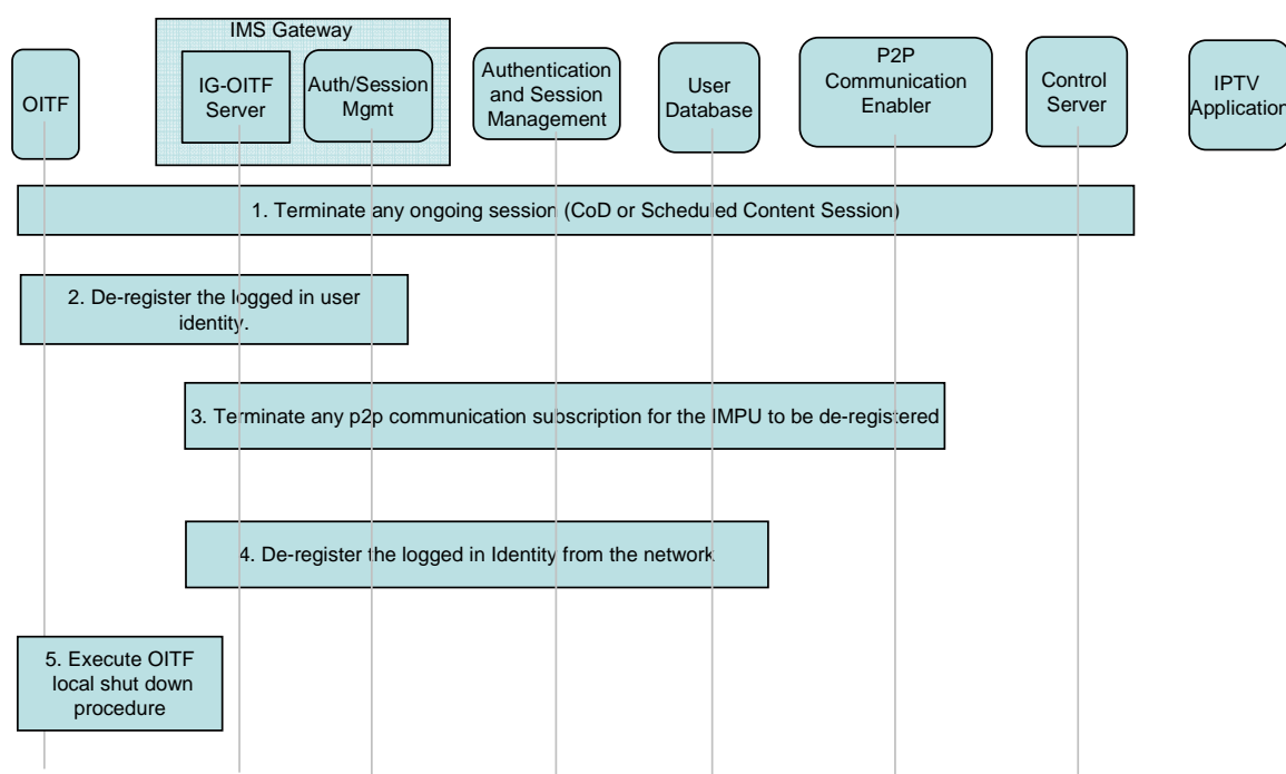
Figure 24: High level Shut-down procedural flow for an OITF
