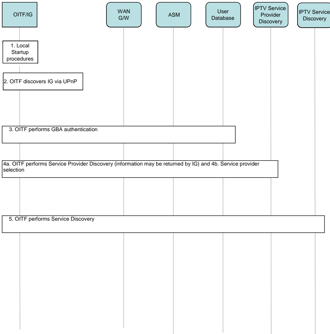
Figure 23: High-level start-up procedural flow for an integrated OITF/IG
