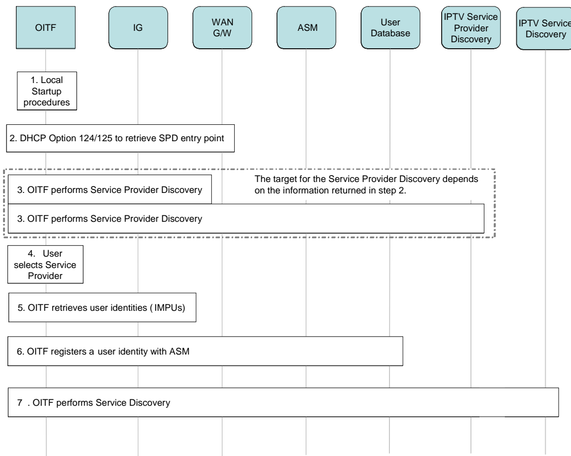
Figure 22: High-level start-up procedural flow for an OITF without native HNI-IGI support
