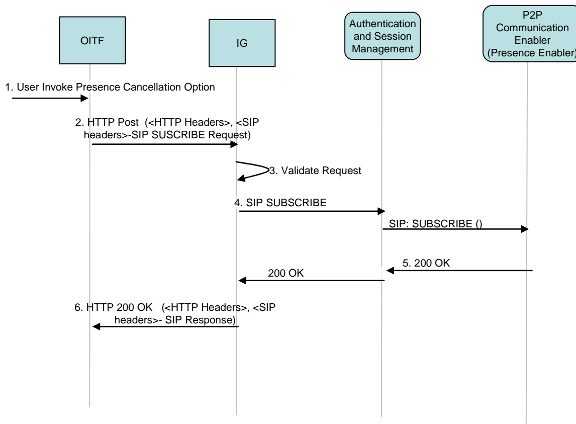
Figure 18: Cancellation of Presence Subscription
