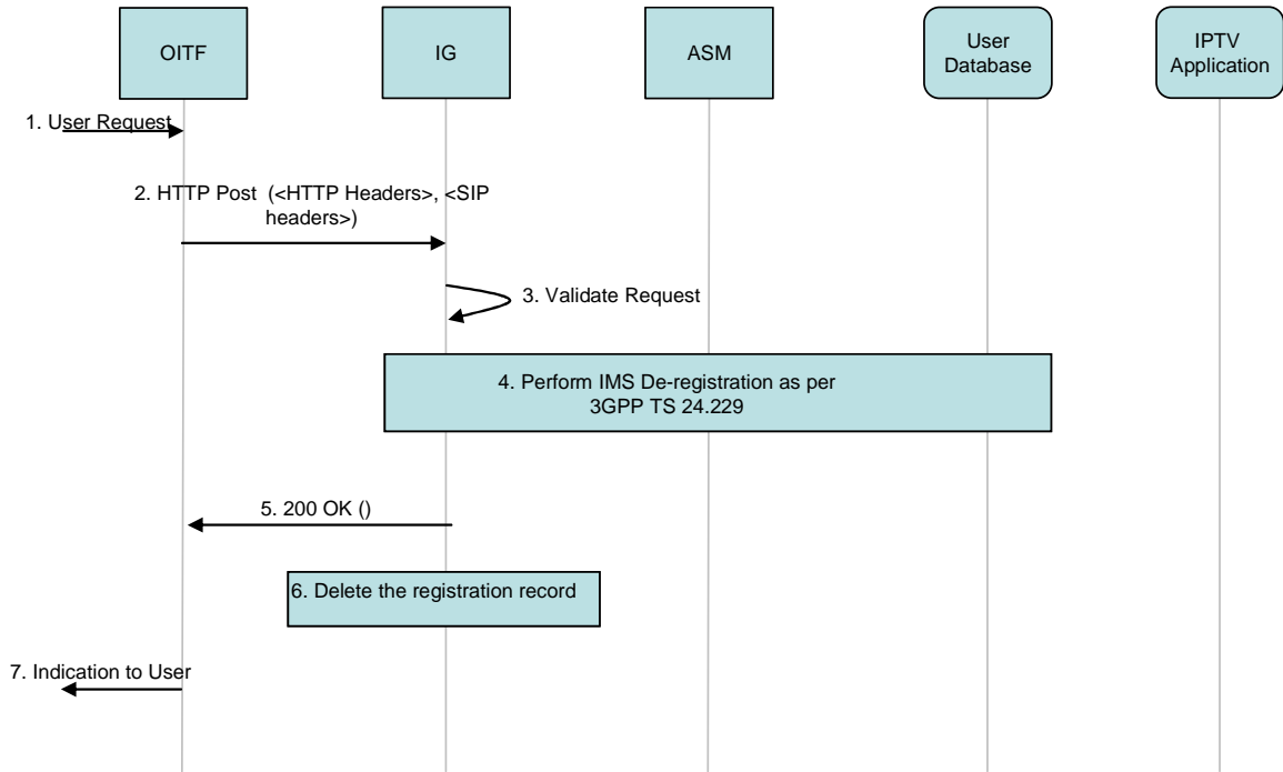
Figure 8: IPTV end-user De-registration procedure in a managed model
