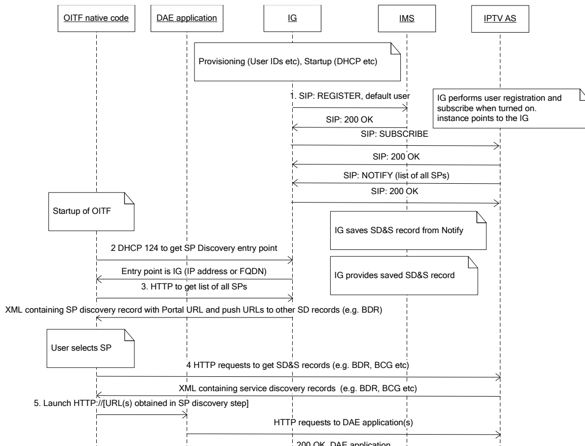
Figure 12: Registration for non-native HNI-IGI
