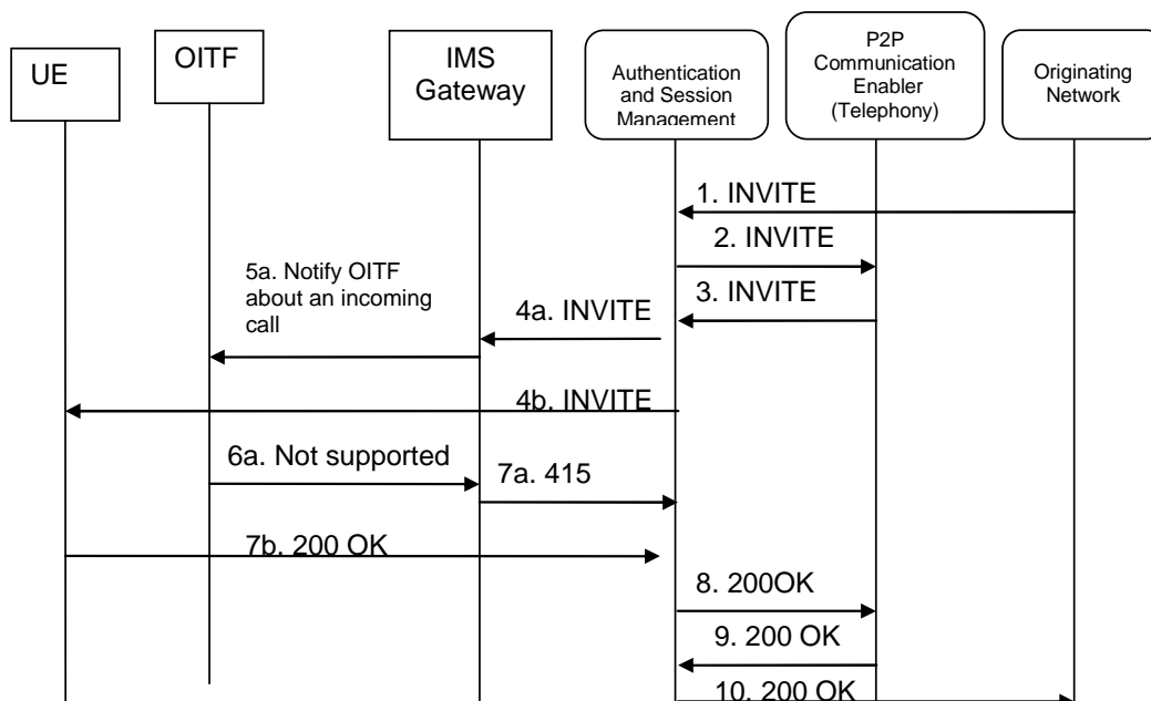
Figure 16: IMS telephony service based caller identification
