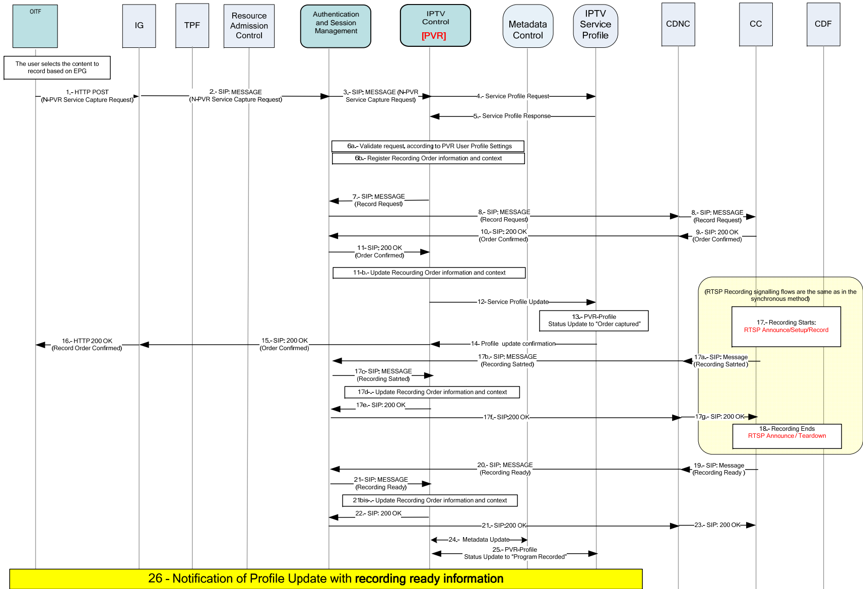
Figure 6-46: Call flow for Network PVR recording - Asynchronous
