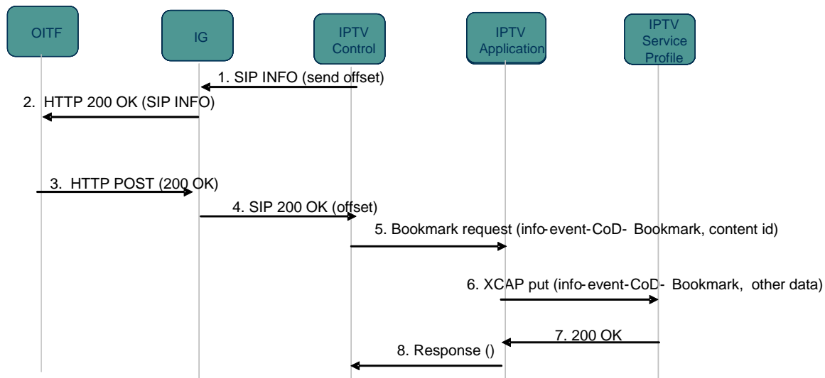
Figure 6-54: Network-initiated Bookmarking
