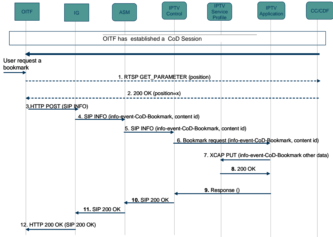
Figure 6-47: IMS-based CoD Bookmark creation and Storage
