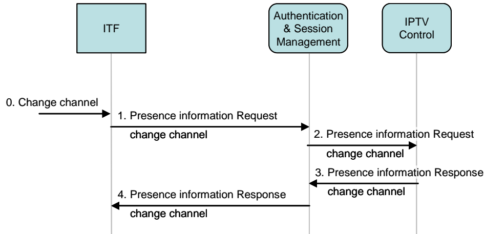
Figure 7-11: Scheduled Content channel switching: Server Side load control
