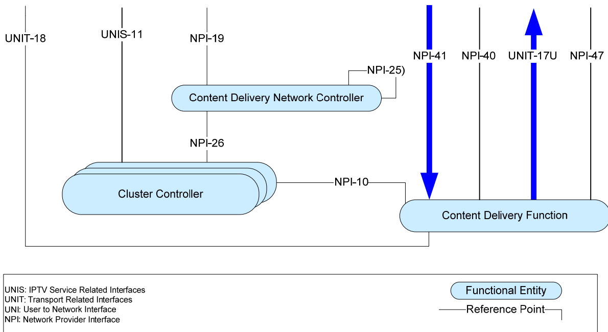
Figure 5-3: CDN Architecture
