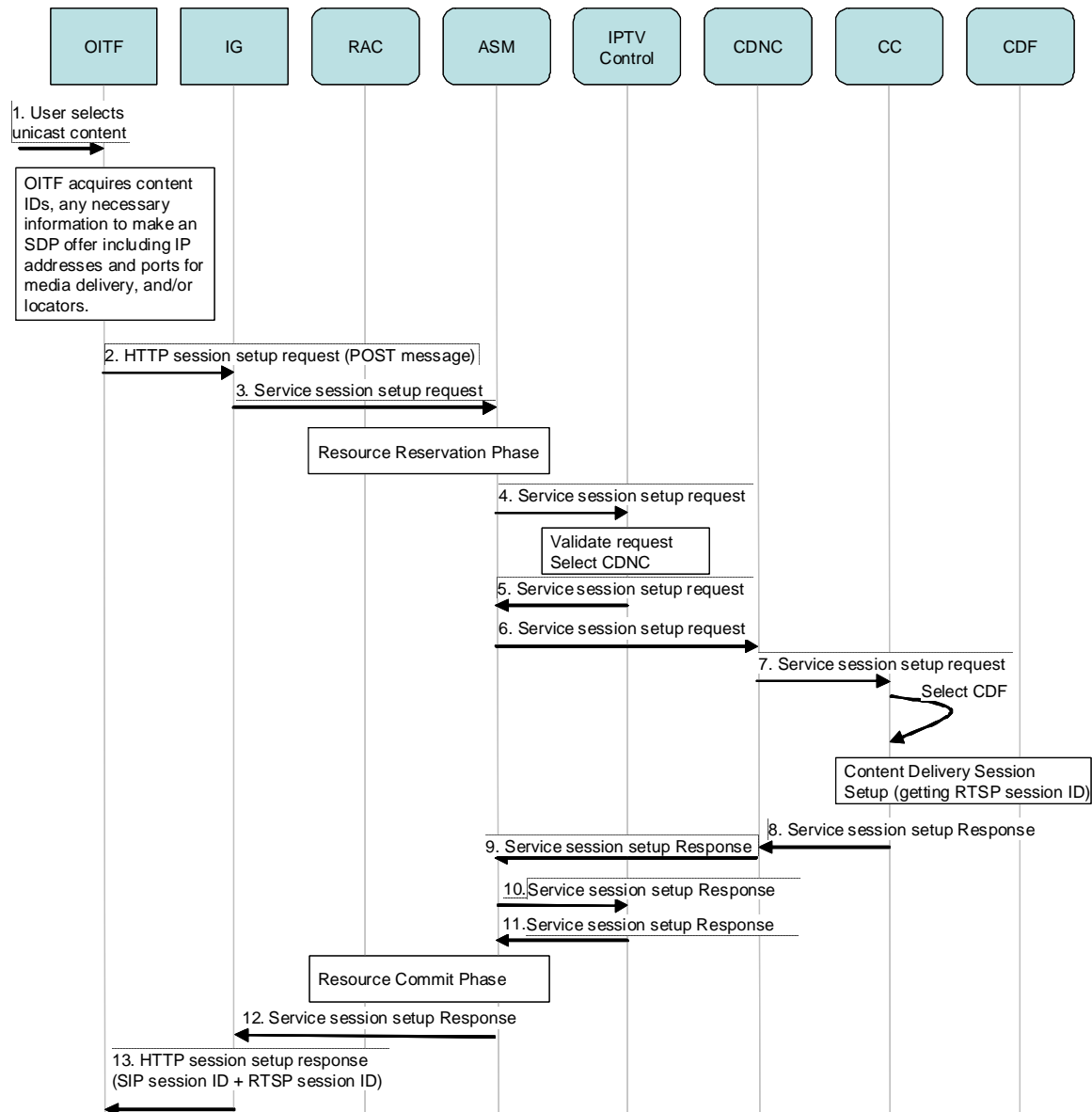
Figure 6-16: Service Session Setup Call Flow
