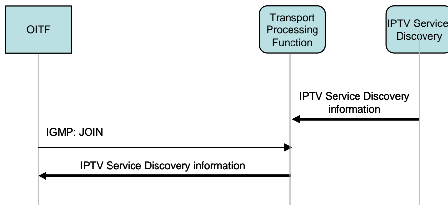
Figure 6-9: Multicast-based IPTV Service Discovery
