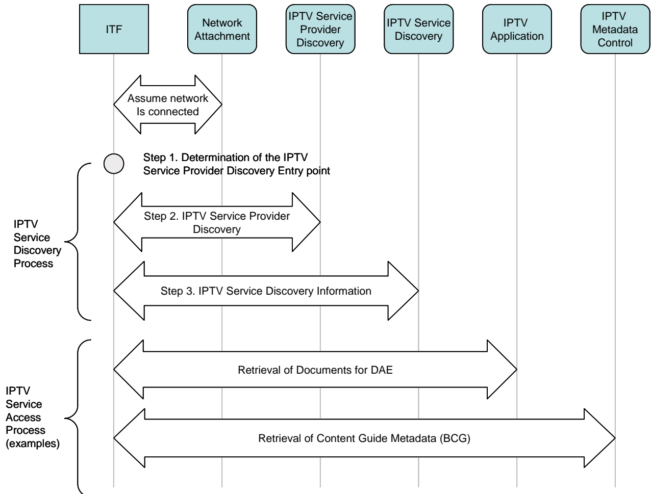
Figure 6-1: High level steps in Service Discovery and Service Access
