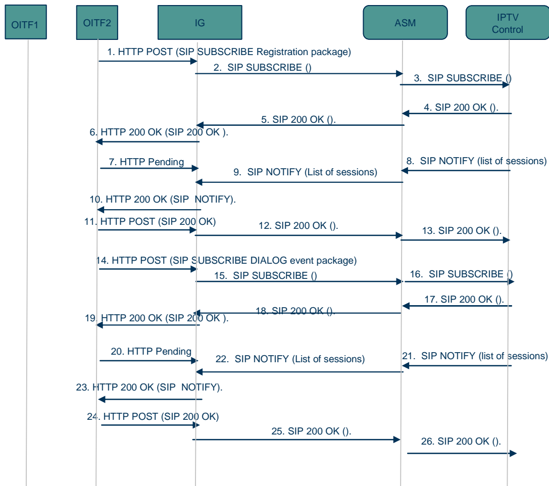
Figure 6-85: Dynamic device discovery and active session awareness
