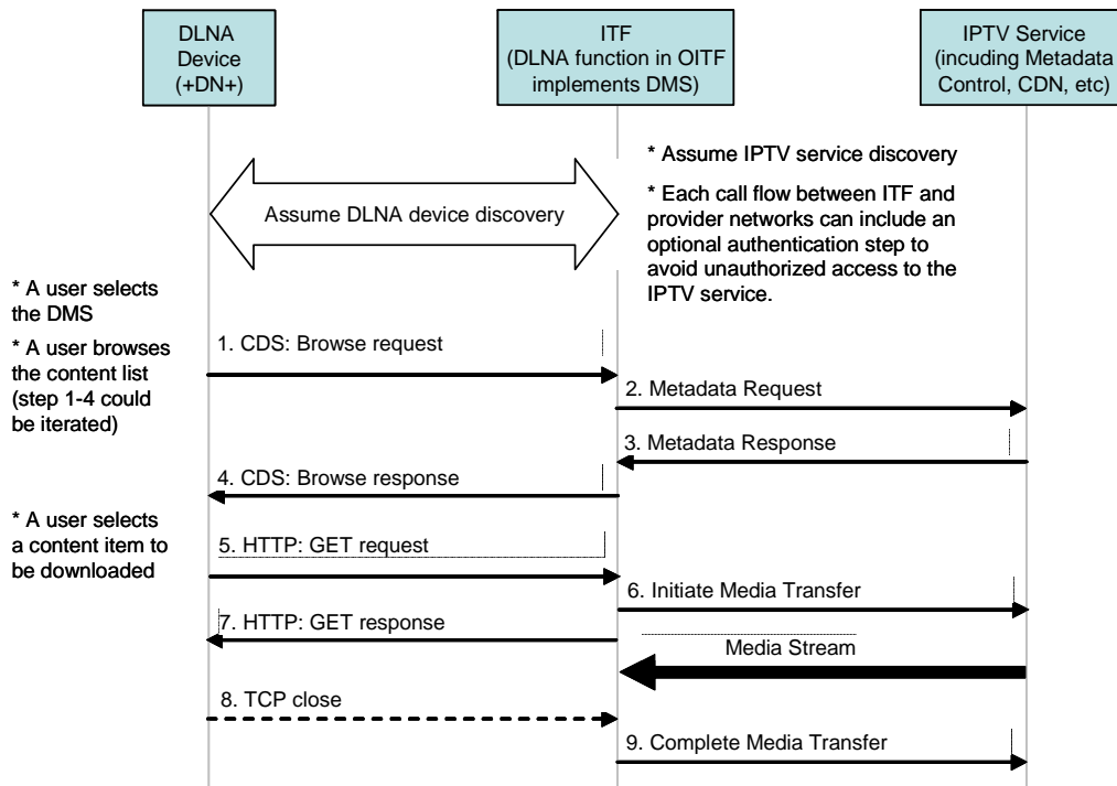
Figure 10-3: Signal flow for DLNA download system
