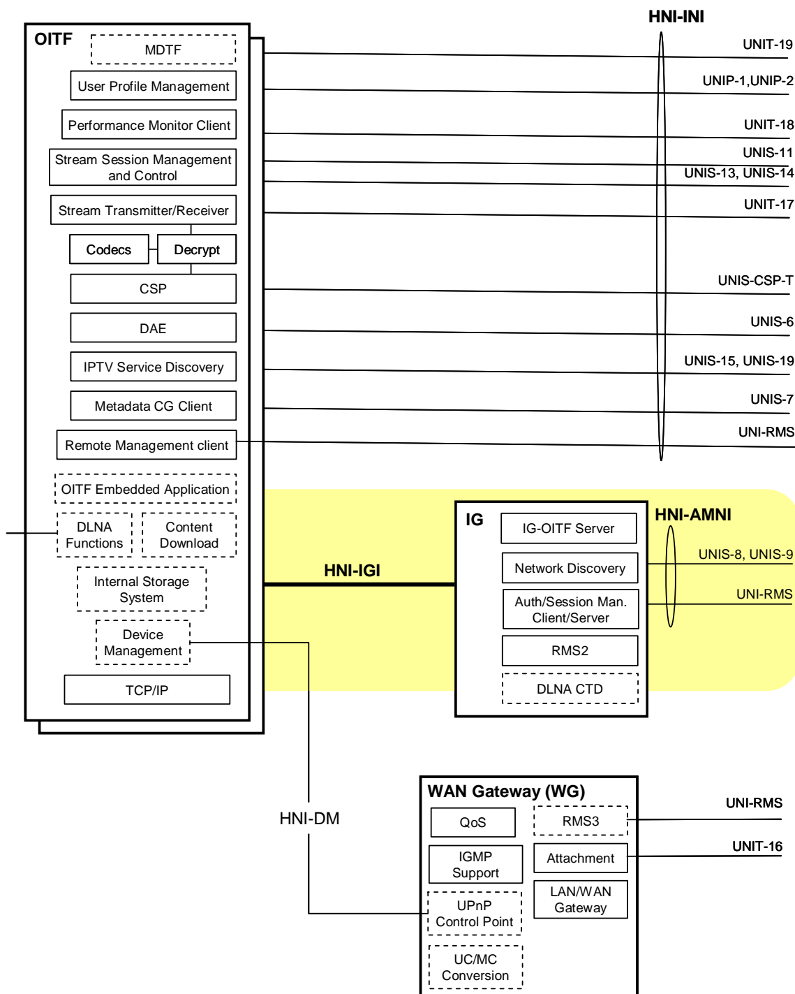
Figure 5-6: OITF and IG
