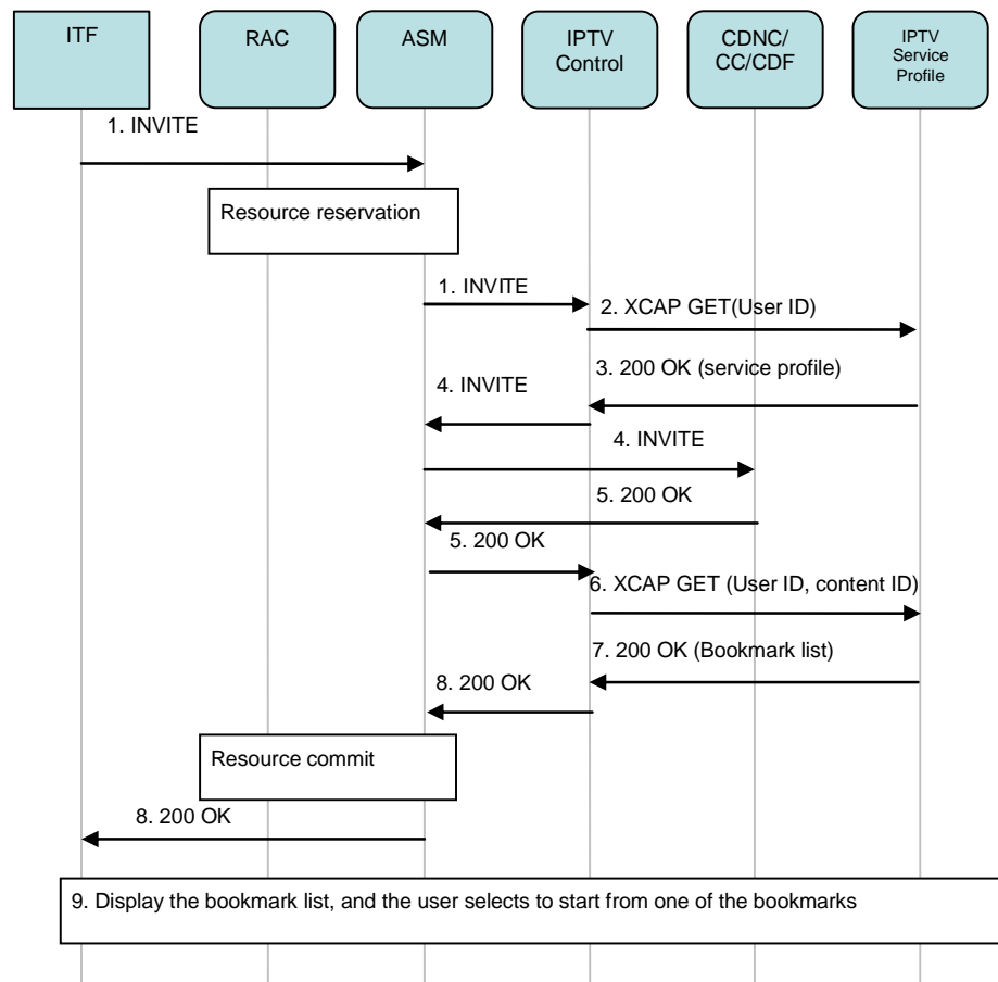
Figure 6-49: Content-related Bookmark Retrieval Call Flow
