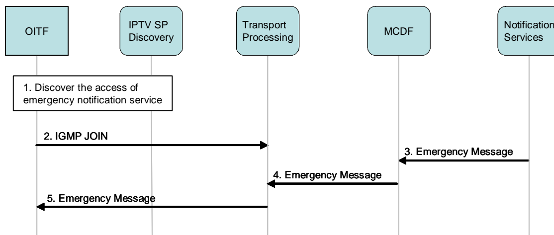
Figure 6-71: Retrieving Emergency notifications
