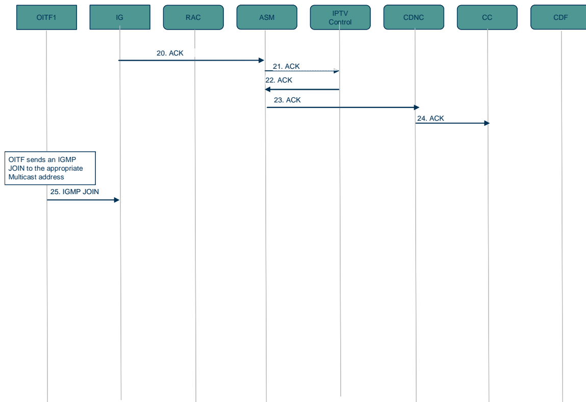
Figure 6-33: Switching from time-shifted to regular Scheduled Content – Part 2
