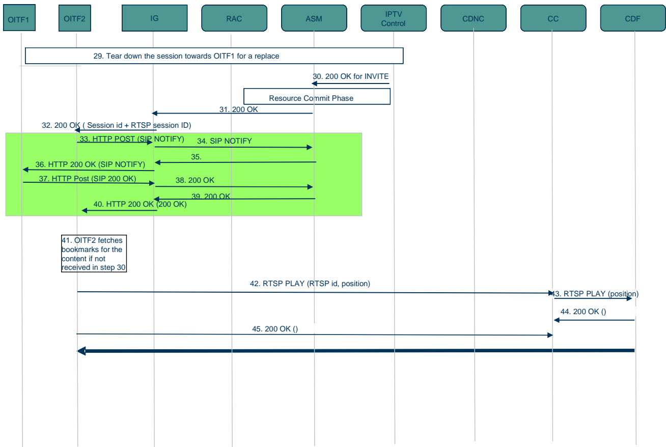
Figure 6-80: Detailed Push procedure for session transfer/replication – Part 2
