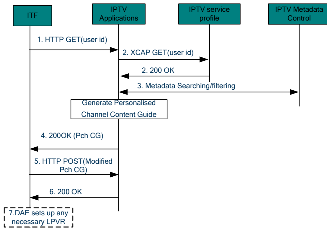
Figure 6-75: Network-centric PCh configuration procedure
