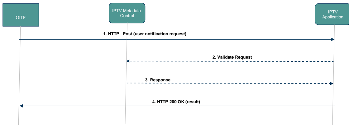
Figure 6-68: DAE procedure for User Notification Services
