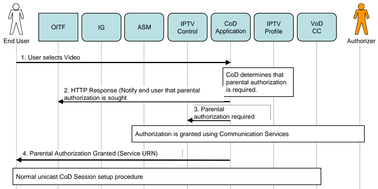
Figure 6-60: Parental Control for browser-based CoD portal application
