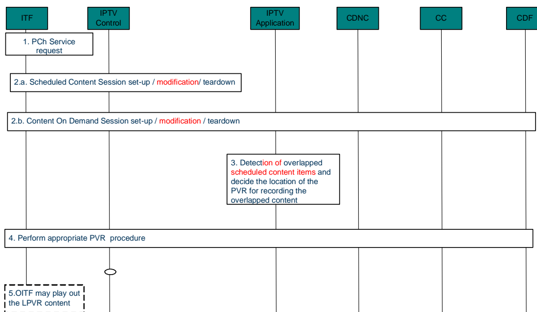
Figure 6-76: Network-centric PCh service set-up procedure
