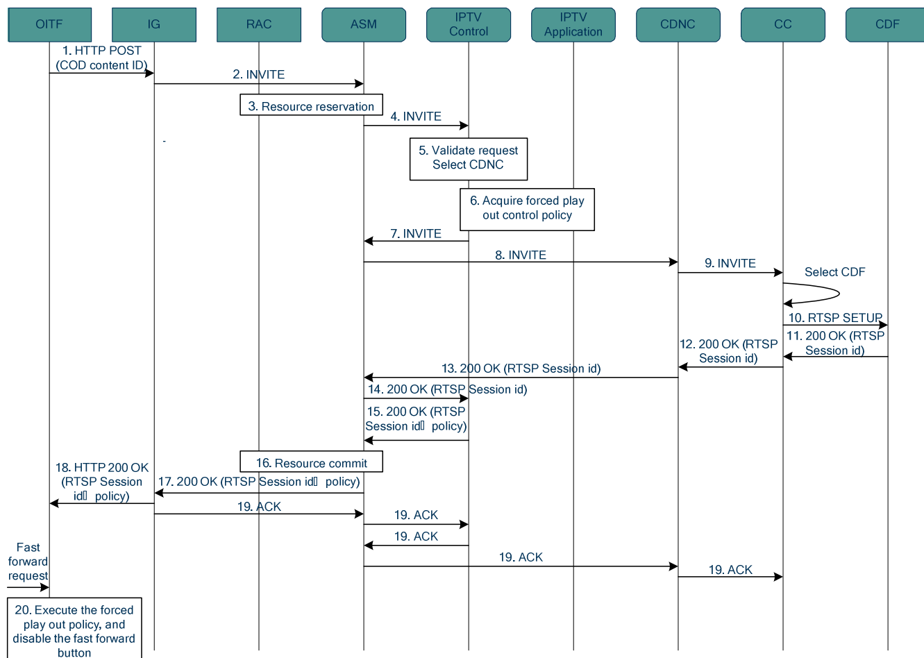
Figure 6-36: Forced Play Out controlled by the OITF
