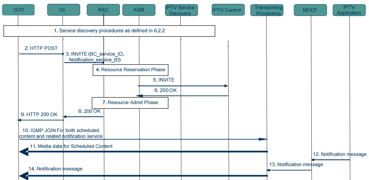
Figure 6-72: Procedure for network-generated Notifications
