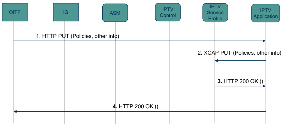
Figure G-5: DAE-based Policy provisioning
