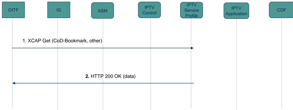
Figure 6-48: IMS-based CoD Bookmark retrieval
