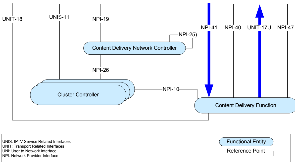
Figure 5-3: CDN Architecture
