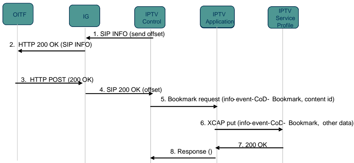
Figure 6-54: Network-initiated Bookmarking
