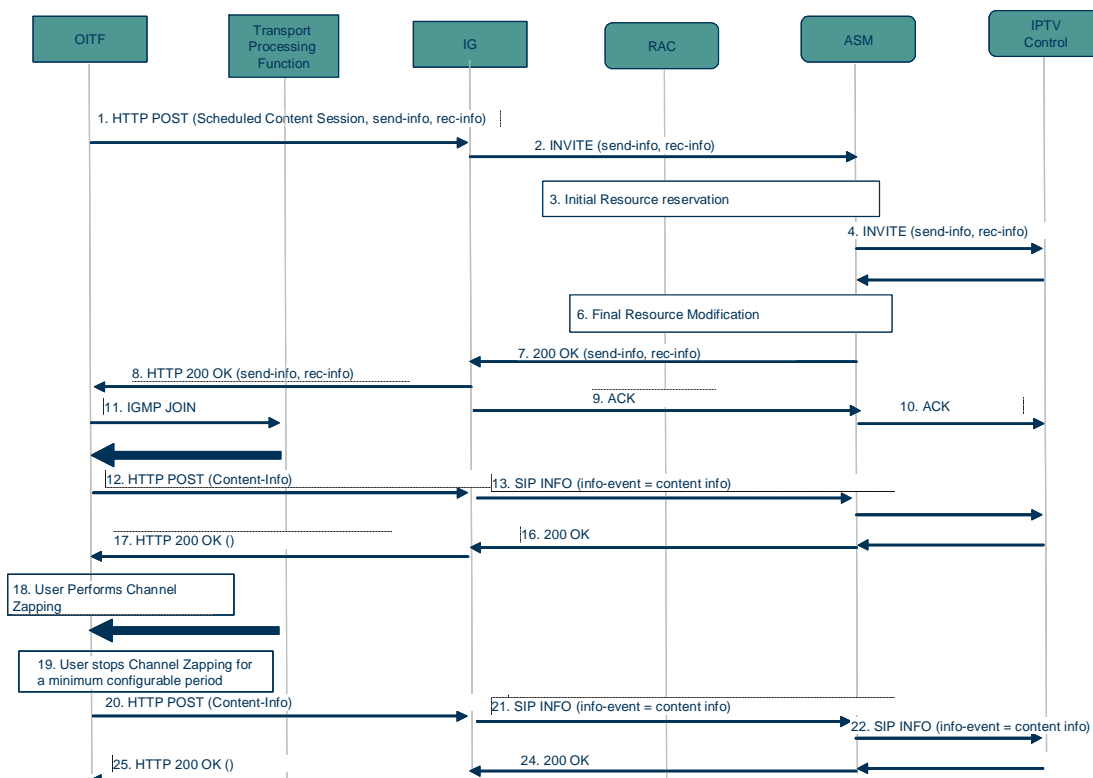
Figure 6-55: Content Reporting at Session initialization
