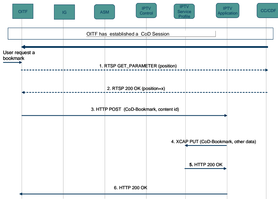
Figure 6-50: DAE-based CoD bookmark creation and storage
