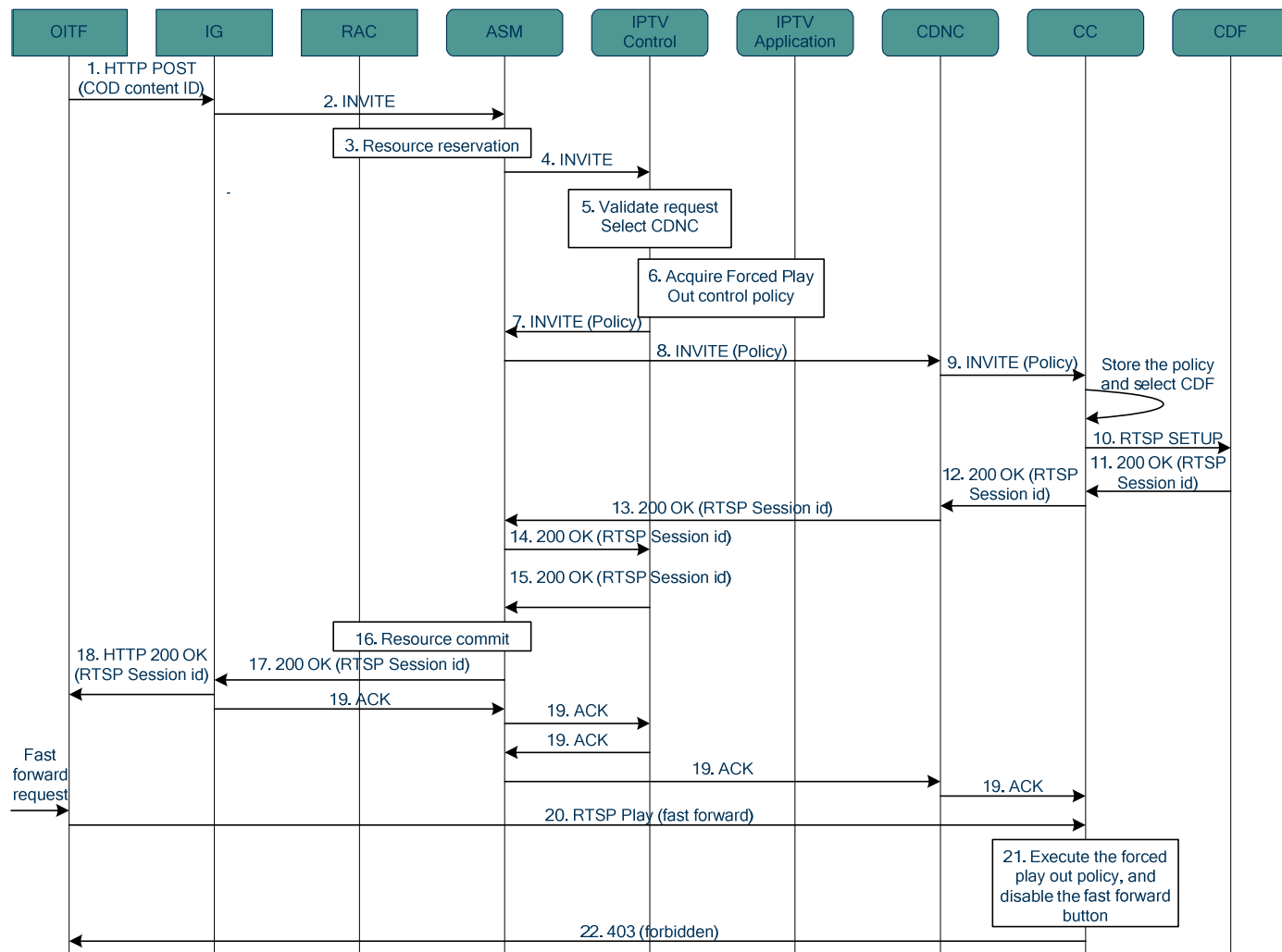
Figure 6-37: Forced Play Out controlled by the CC
