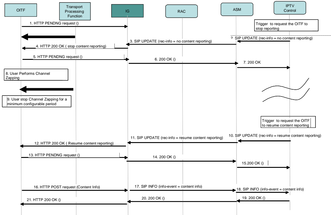
Figure 6-56: Mid-session signalling for content reporting
