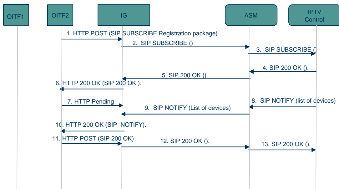
Figure 6-81: Dynamic Discovery of devices
