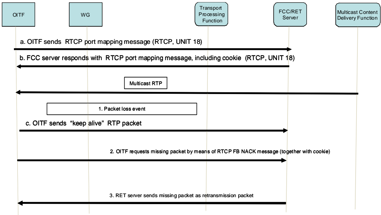
Figure 14: Port mapping process and keep-alive packets for RET
