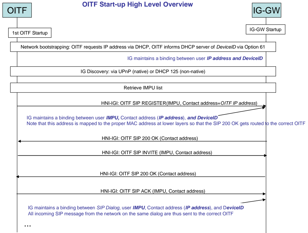
Figure 12: Overview of OITF Startup
