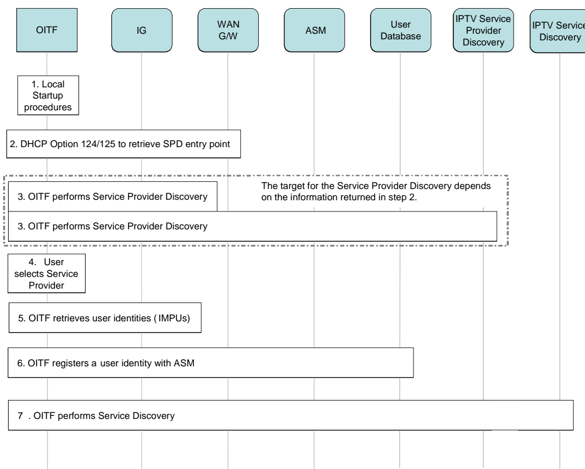
Figure 9: High-level start-up procedural flow for an OITF without native HNI-IGI support
