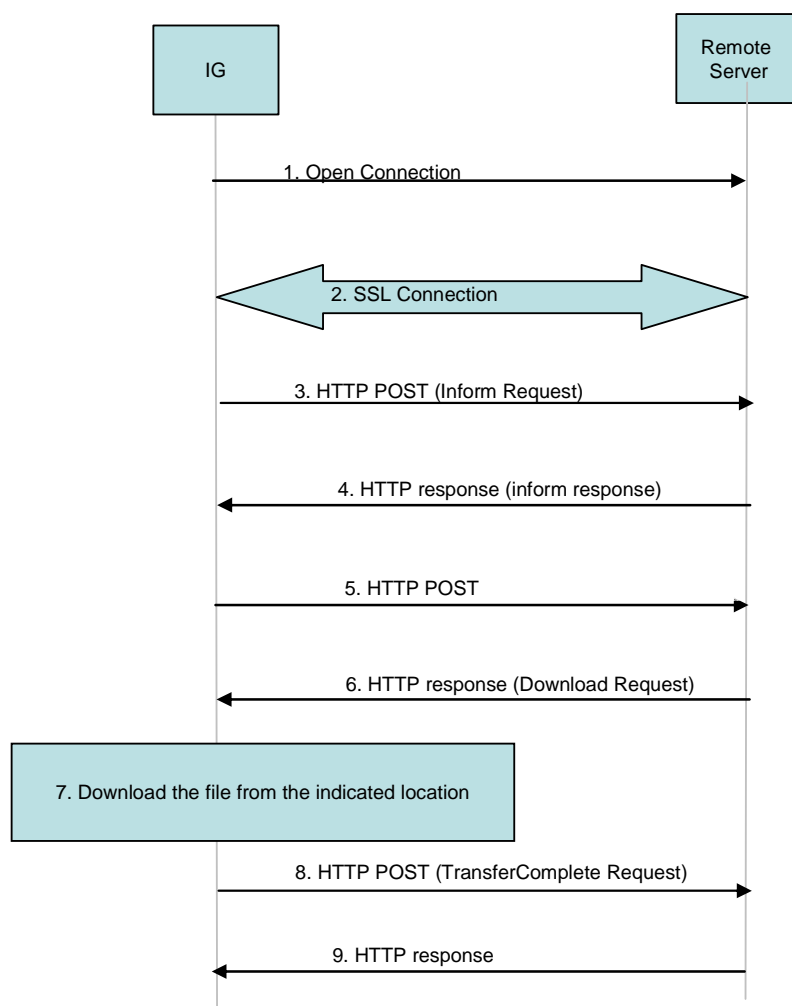
Figure 6: Sequence for the Configuration of an IG
