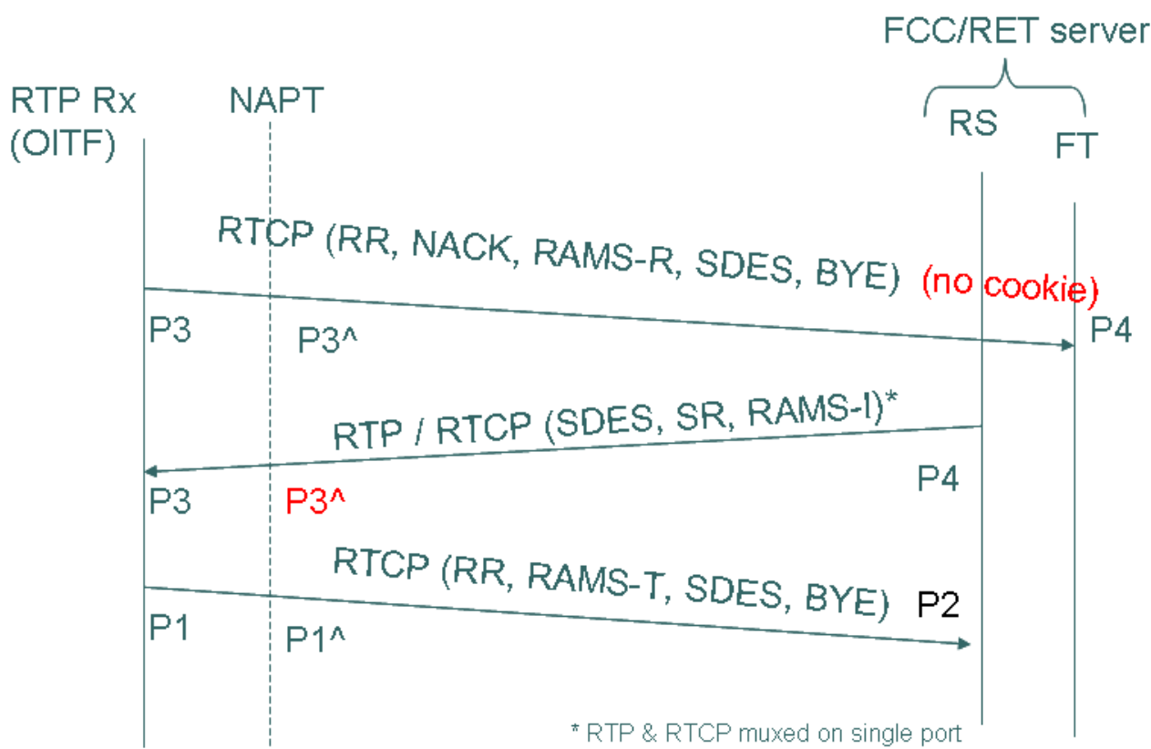
Figure 16: NAT traversal for FCC/RET without cookie signalling
