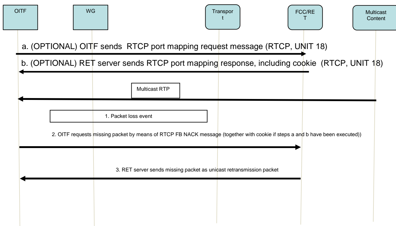
Figure 18: Call flow for Scheduled Content with unicast retransmission service
