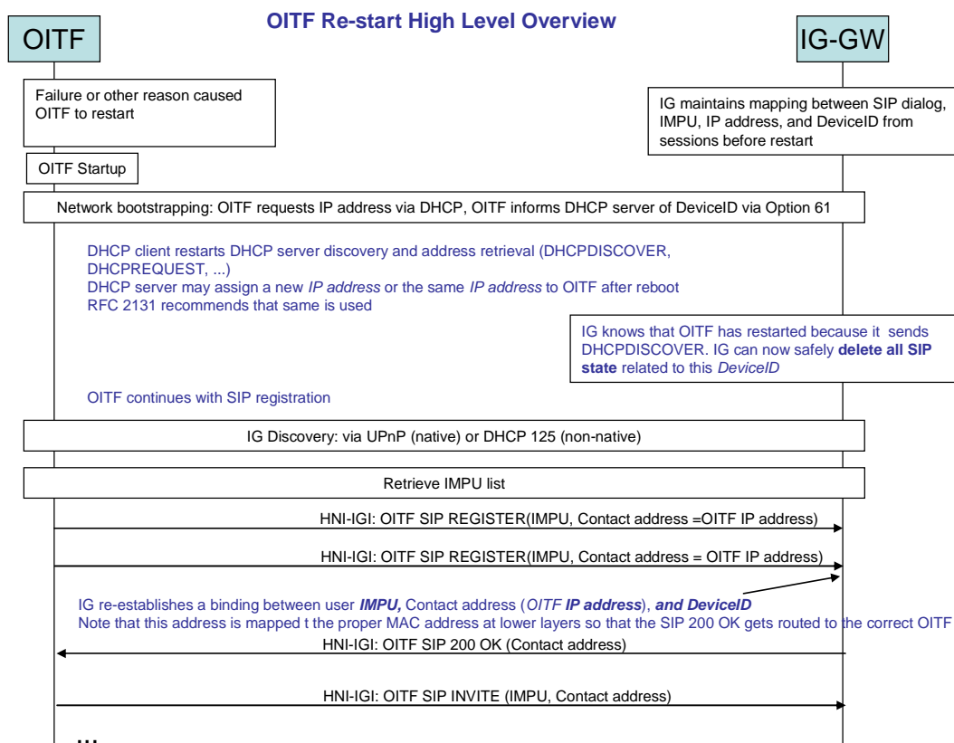
Figure 13: Overview of OITF Restart
