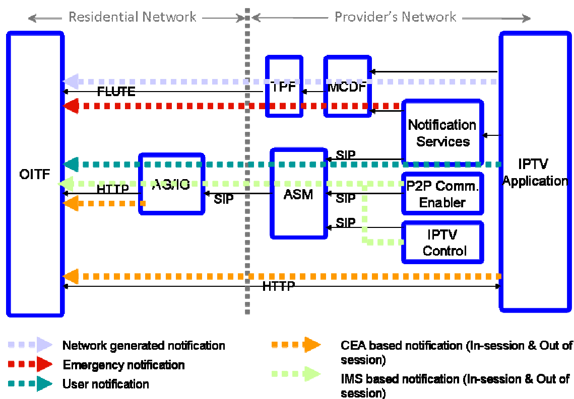
Figure 17: Overview of notification services
