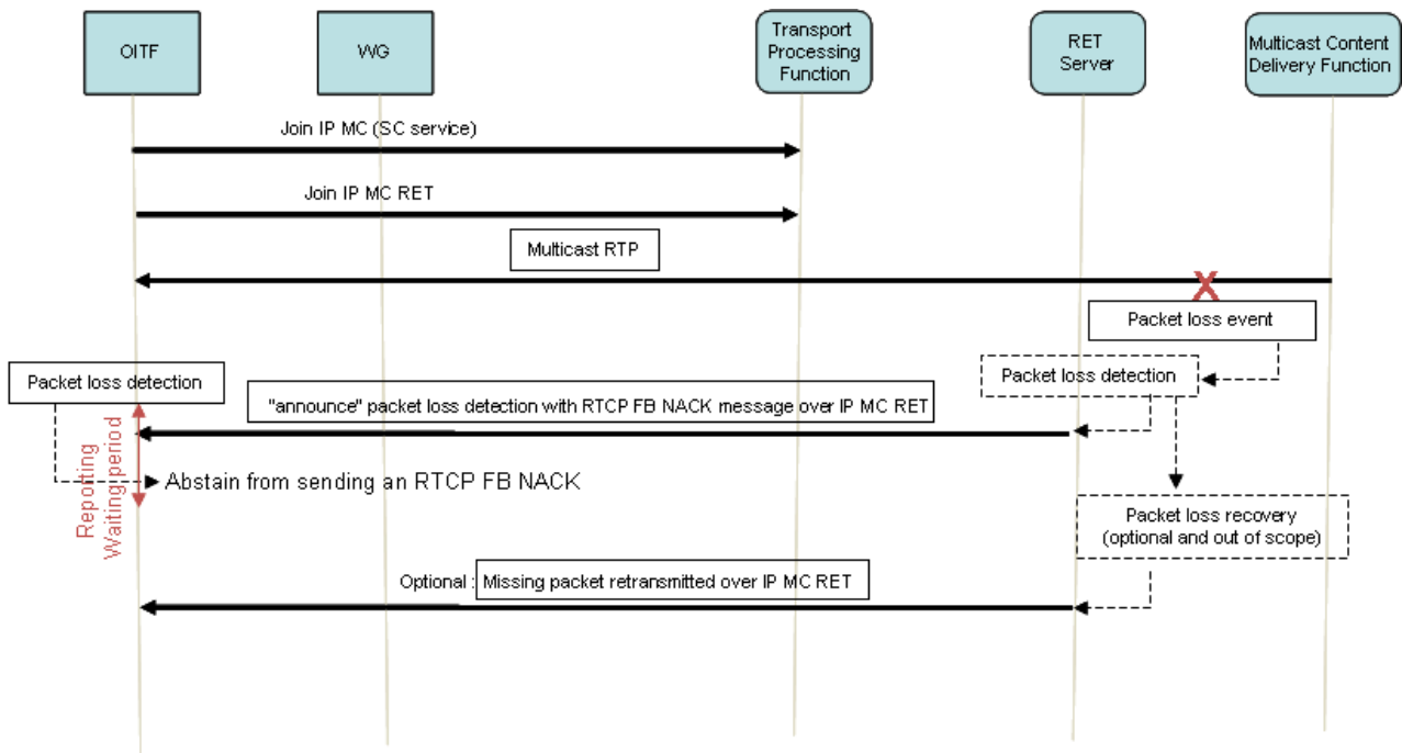
Figure 20: MC RET protocol interaction for packet loss upstream of RET server
