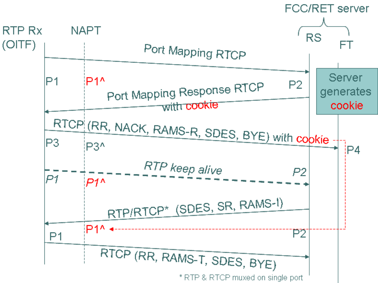
Figure 15: NATP traversal for FCC/RET with cookie signaling
