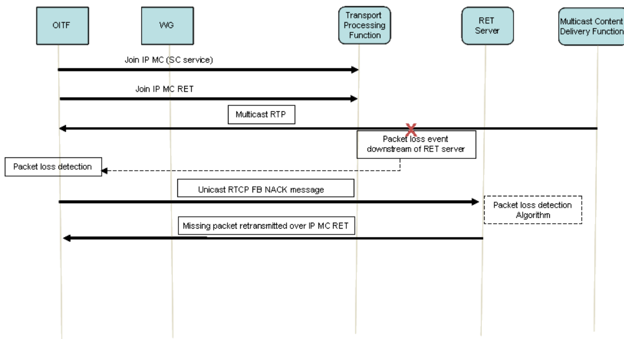
Figure 21: MC RET protocol interaction for packet loss downstream of RET server, with the OITF acting as immediate reporter
