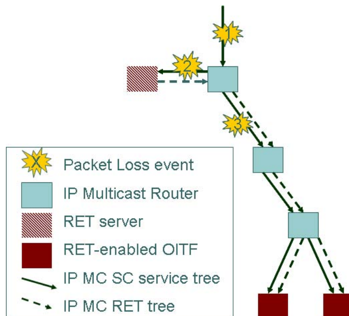
Figure 19: Example showing location of packet loss deep in the network relative to the RET server
