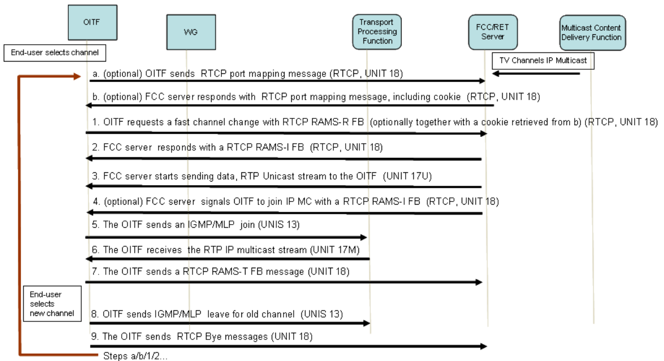
Figure 22: Call flow for Fast Channel Change Service
