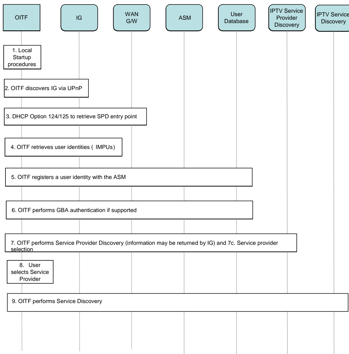
Figure 8: High level Start up procedural flow for an OITF with native HNI-IGI support
