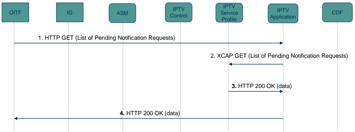
Figure 17: DAE-based fetching of Pending Notification Requests
